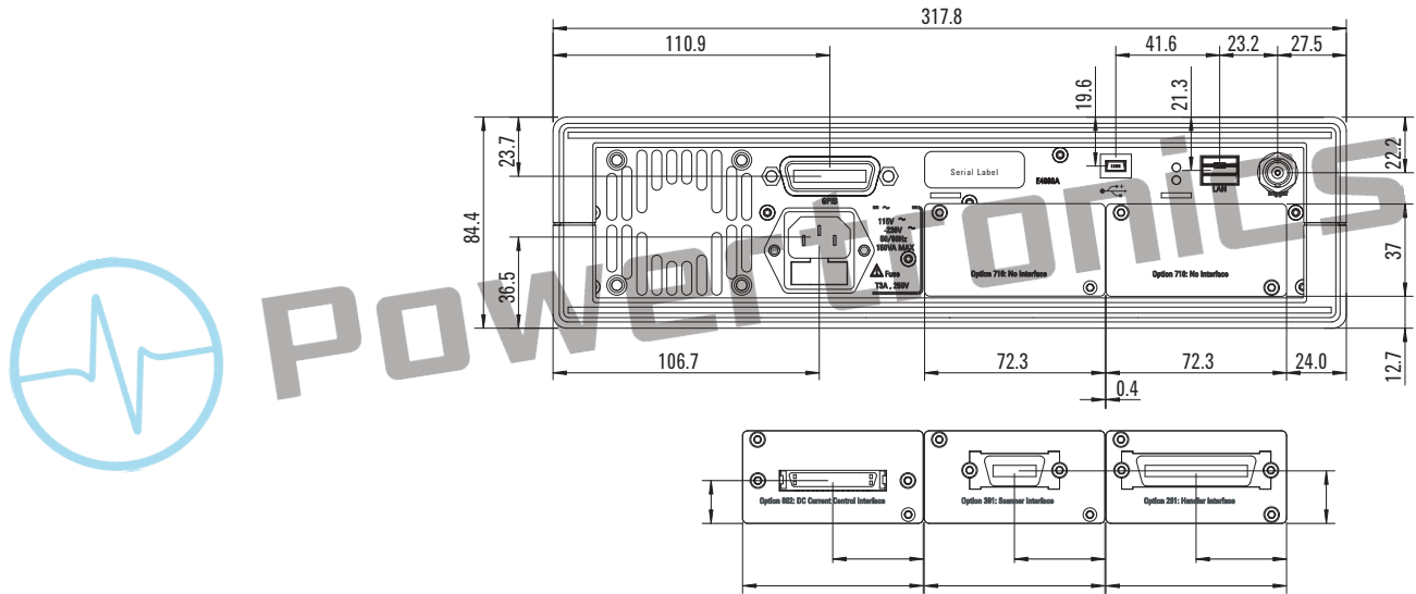
Figure 5. Dimensions (rear view, with handle and bumper, in millimeters, nominal)
