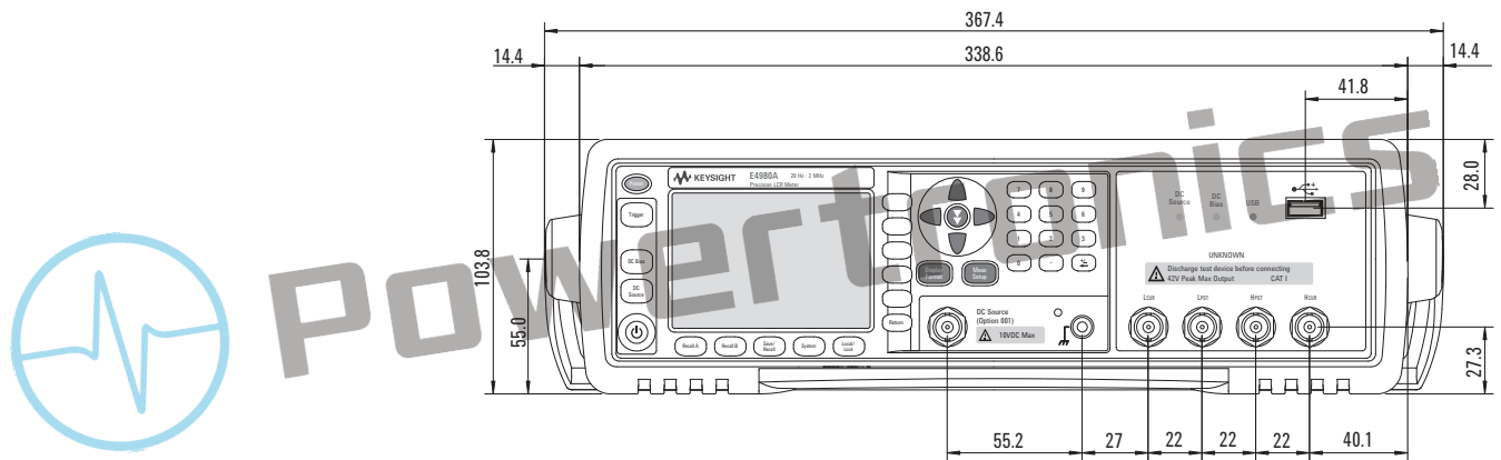
Figure 2. Dimensions (front view, with handle and bumper, in millimeters, nominal)
